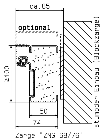
Zarge "ZNG 68/76"
