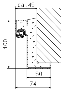
Hauptzarge "ZG 68/76"
